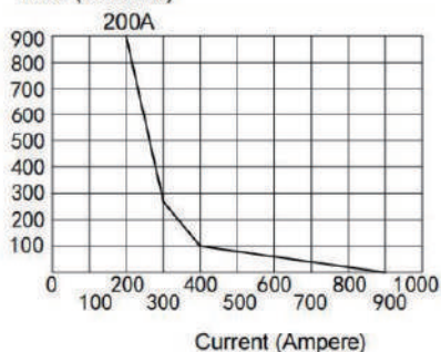
Contact Current Plot Time (Seconds)
