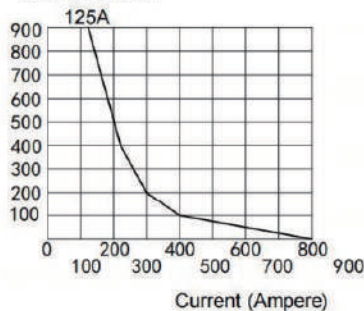
Contact Current Plot Time (Seconds)
