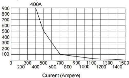
Contact Current Plot Time (Seconds)
