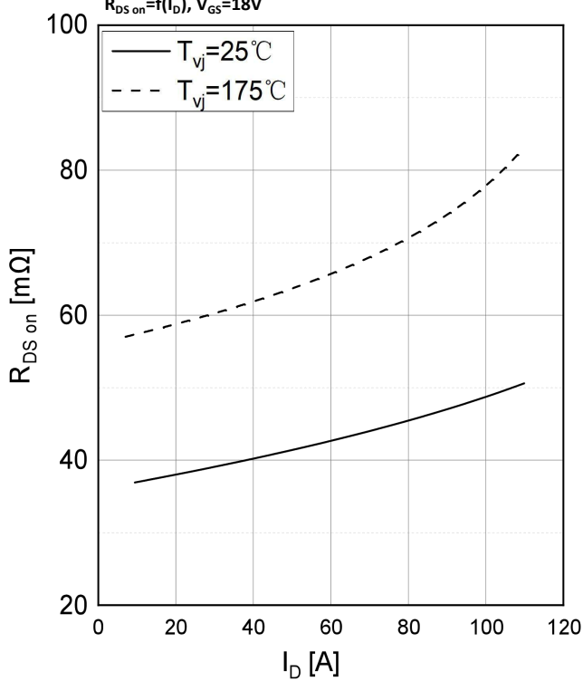
导通电阻 On-Resistance R_{DS\text{ on}} = f(I_D), V_{GS} = 18\text{V}
