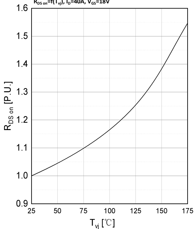
标准化导通电阻 Normalized On-Resistance R_{DS\text{ on}} = f(T_{vj}), I_D = 40\text{A}, V_{GS} = 18\text{V}
