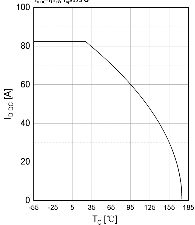
连续漏极电流衰减
