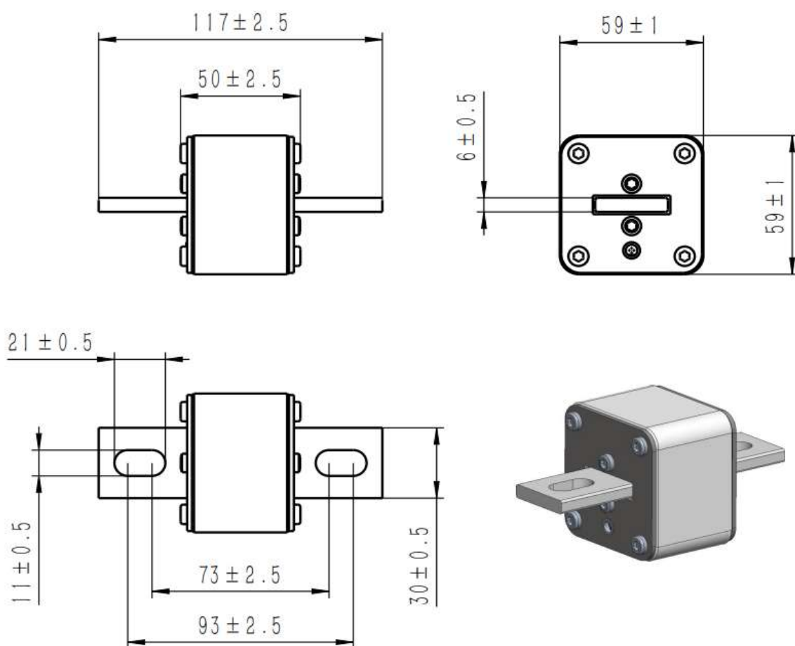
Bolted: xxxBN-59E 长条螺栓横向安装 without fuse indicator
