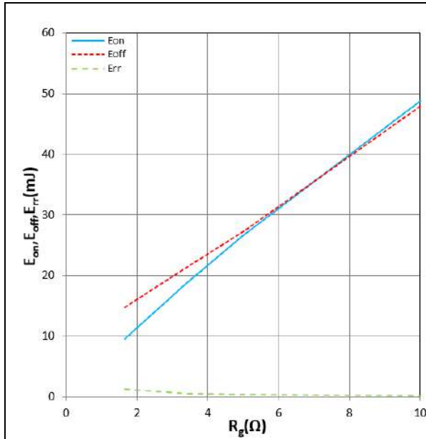
Figure 13. E_{on} , E_{off} , E_{rr} vs R_g
