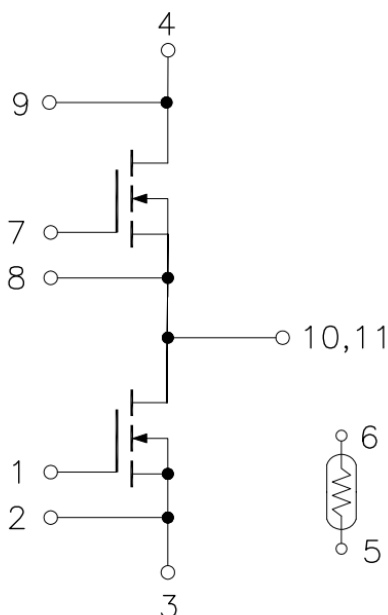
Figure 1. Out drawing & circuit diagram for HCS600FH120D3C1
