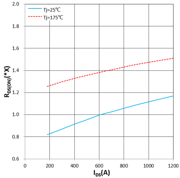
Figure 10. R_{DS(ON)} vs I_{DS} T_J=25/175^\circ C , V_{GS}=+18V , 1.0X=3.2m\Omega
