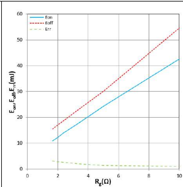
Figure 14. E_{on} , E_{off} , E_{rr} vs R_g
