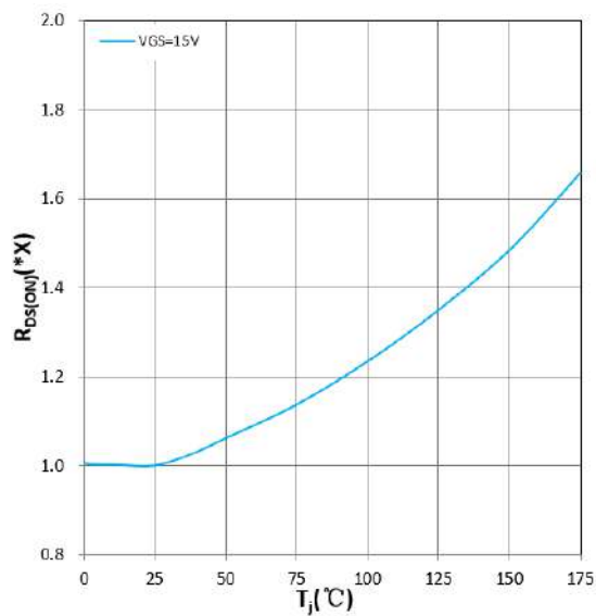
Figure 8. R_{DS(ON)} VS T_J V_{GS}=+15\text{V} , I_D=540\text{A} , 1.0\text{X}=3.5\text{m}\Omega
