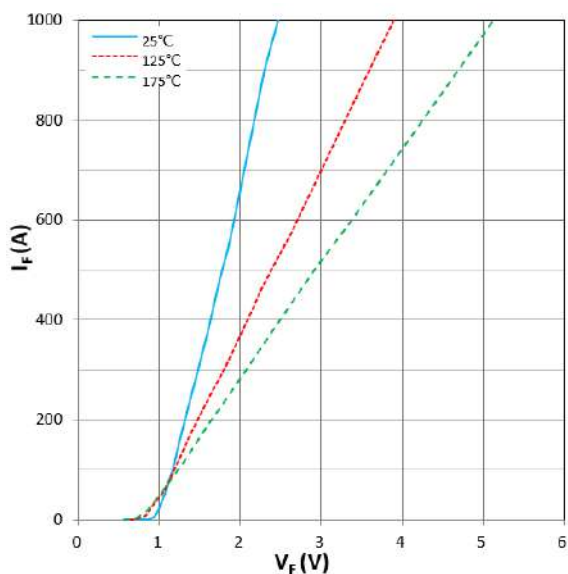
Figure 7. I_F VS V_F V_{GS}=0\text{V}
