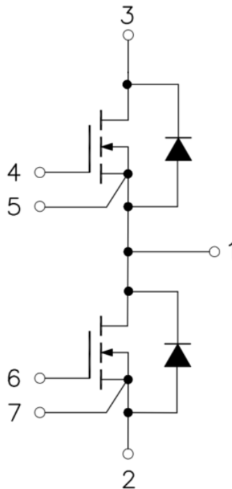
Figure 1. Out Drawing & Circuit Diagram HCS540FH120A2A1
