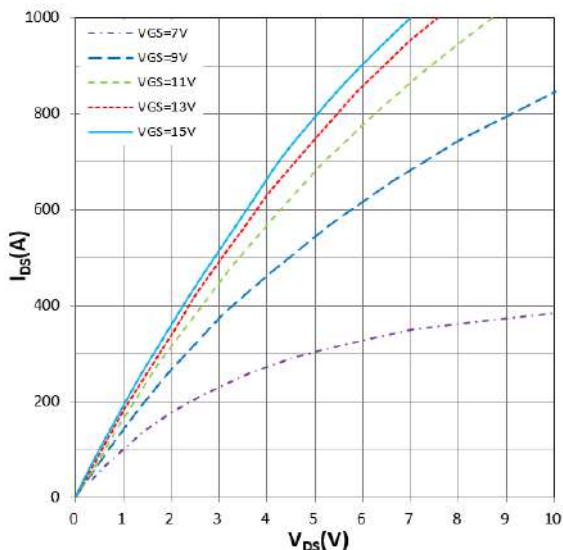
Figure 6. I_{DS} VS V_{DS} T_J=175^{\circ}\text{C}
