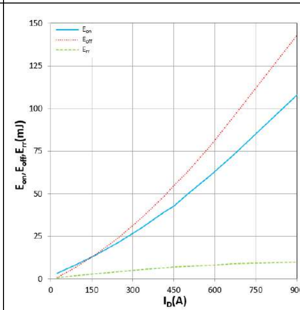
Figure 16. Eon, Eoff, Err vs ID
