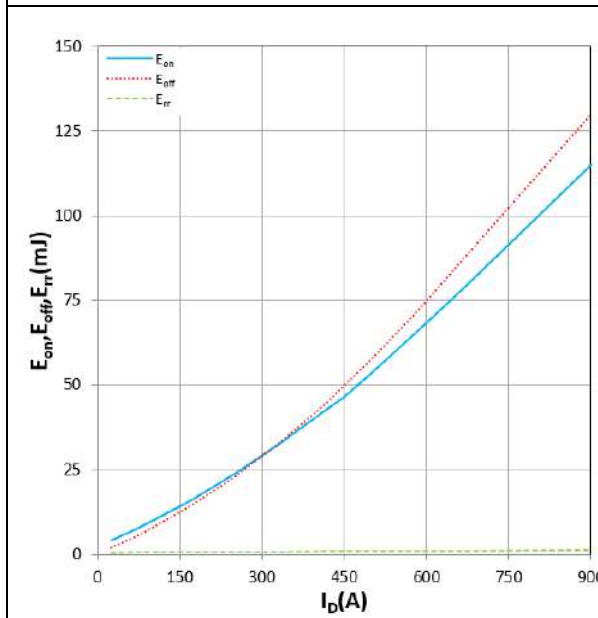
Figure 15. Eon, Eoff, Err vs ID
