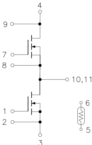
Figure 1. Out drawing & circuit diagram for HCS450FH170D3C1
