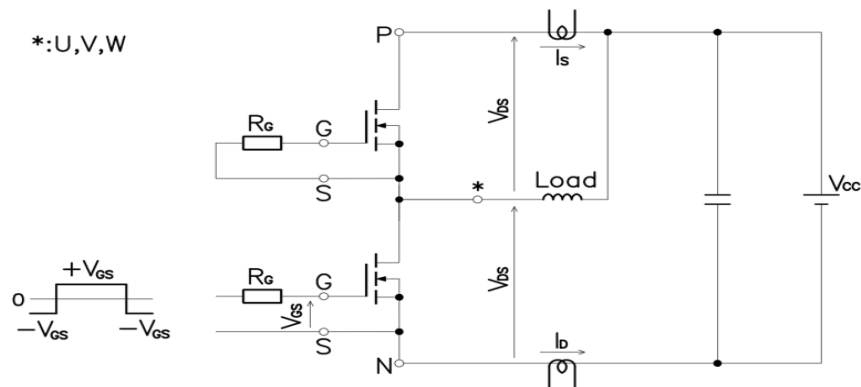
Figure 3. Switching Time Measure Circuit
