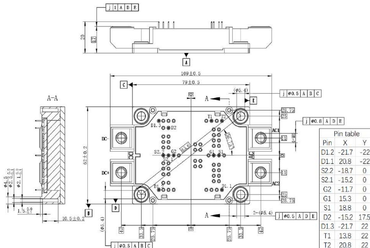
Figure 2. Physical Dimensions
