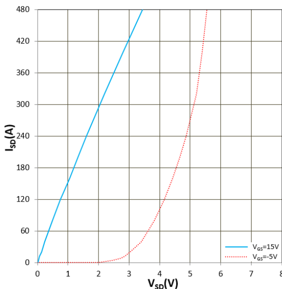
Figure 8. I_{SD} VS V_{SD}(V_F) T_J = 175^\circ\text{C}
