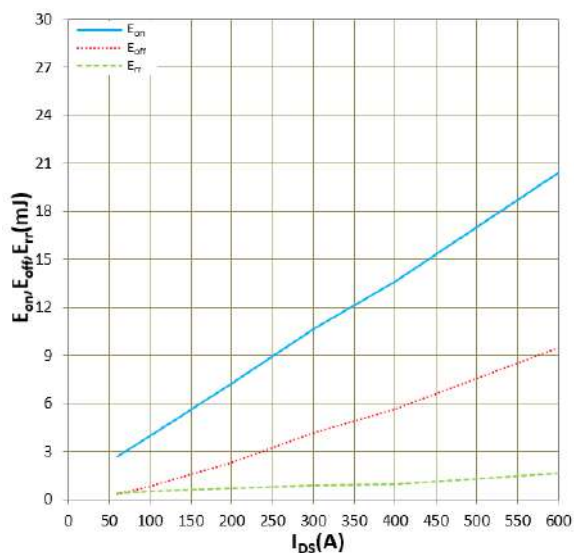
Figure 15. E_{on} , E_{off} , E_{rr} VS I_{DS} T_j=25^{\circ}\text{C} , V_{CC}=600\text{V} , V_{GS}=+15\text{V}/-4\text{V} R_{G(ON)}R_{G(OFF)}=5.1/3.3\Omega , Inductive Load
