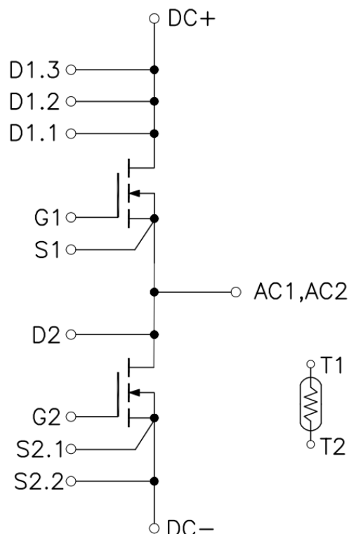
Figure 1. Out Drawing & Circuit Diagram HCS400FH120D4C2
