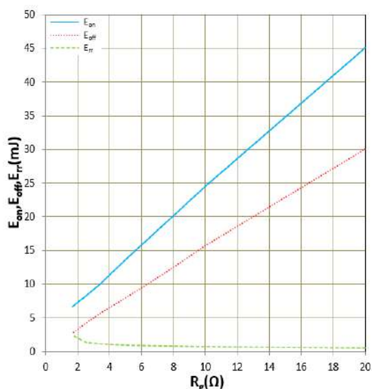
Figure 13. E_{on} , E_{off} , E_{rr} VS R_g T_j=25^{\circ}\text{C} , V_{CC}=600\text{V} , I_D=400\text{A} , V_{GS}=+15\text{V}/-4\text{V} Inductive Load
