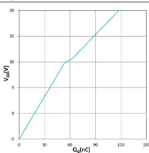
Figure 16. V_{GS} vs Q_G V_{DD} = 800\text{V} , I_D = 40\text{A}
