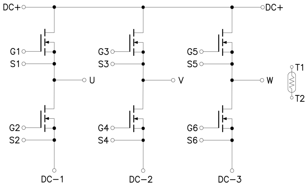
Figure 1. Out drawing & circuit diagram for HCS36FT140E1Q1
