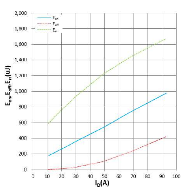
Figure 14. E_{on} , E_{off} , E_{tr} vs I_D T_j = 150^{\circ}\text{C} , V_{DD} = 800\text{V} , R_G = 5.1\text{m}\Omega , V_{GS} = +18/-4\text{V}
