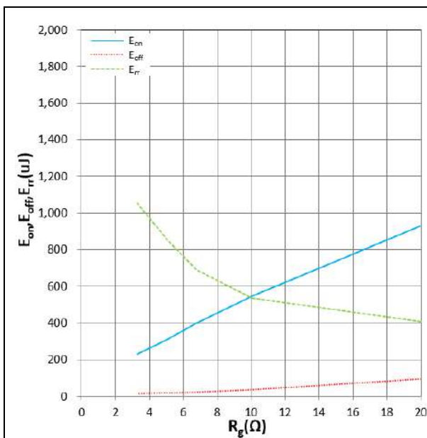
Figure 13. E_{on} , E_{off} , E_{tr} vs R_G T_j = 150^{\circ}\text{C} , V_{DD} = 800\text{V} , I_D = 25\text{A} , V_{GS} = +18/-4\text{V}
