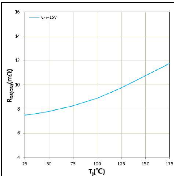
Figure 9. R_{DS(ON)} vs T_J I_D = 160A
