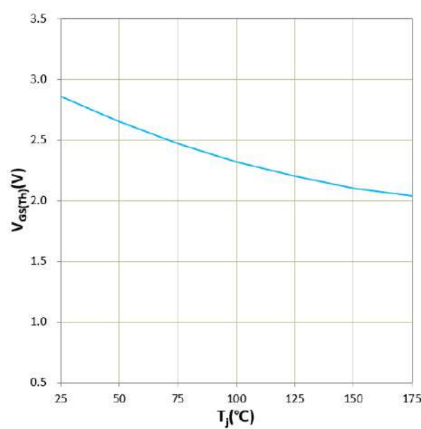
Figure 12. V_{GS(TH)} vs T_J V_{GS} = V_{DS} , I_D = 54mA
