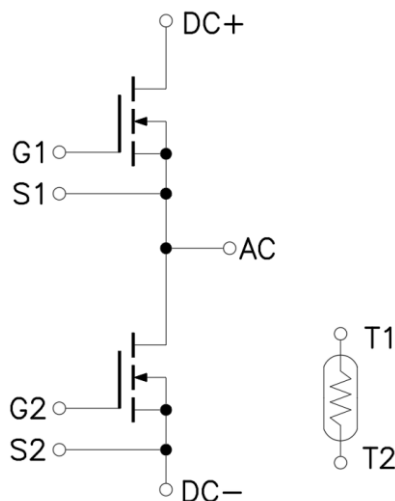
Figure 1. Out drawing & circuit diagram for HCS08FH120E2A2
