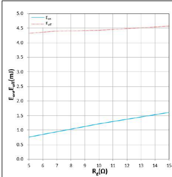
Figure 13. E_{on} , E_{off} vs R_g (Typ) V_{CC}=700V , I_C=50A , V_{GE}=+15V/-8V , T_j=125^\circ C Inductive Load
