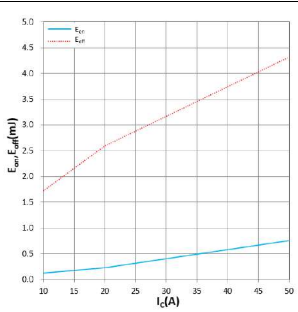
Figure 14. E_{on} , E_{off} vs I_C (Typ) V_{CC}=700V , R_G=5\Omega , V_{GE}=+15V/-8V , T_j=125^\circ C Inductive Load
