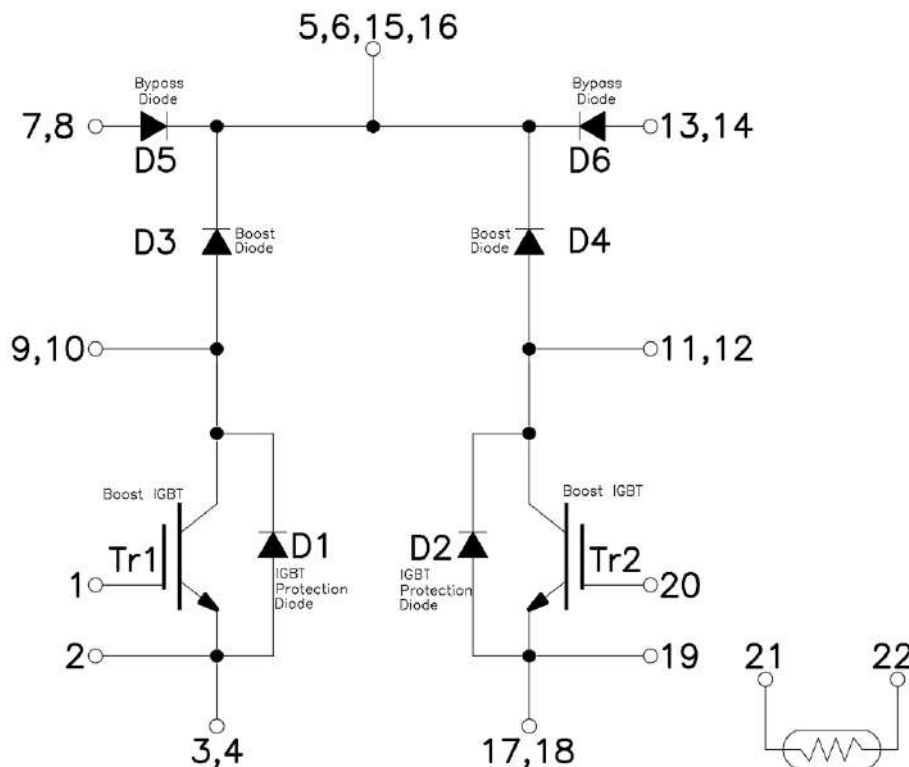
Figure 1. Out drawing & circuit diagram for HCF50FB120F0H1
