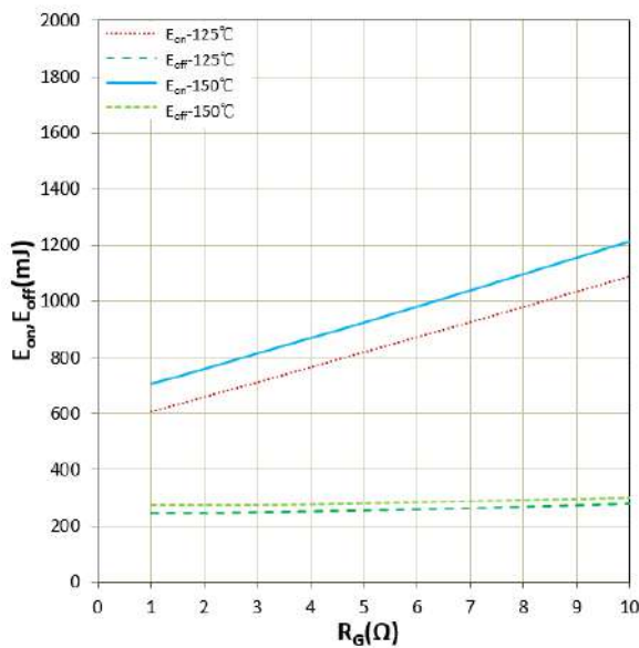
Figure 9. E_{on} , E_{off} vs R_G (Typ) V_{CC}=900\text{V} , V_{GE}=+15\text{V}/-8\text{V} , I_C = 800\text{A} Inductive Load
