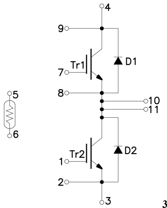
Figure 1. Out drawing & circuit diagram for HCG800FH170D3RE2
