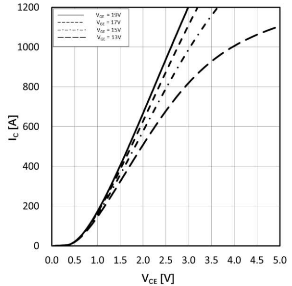
Fig.2 Typical Output Characteristic,IGBT,Inverter I_c = f(V_{CE}) T_{vj} = 175^{\circ}C
