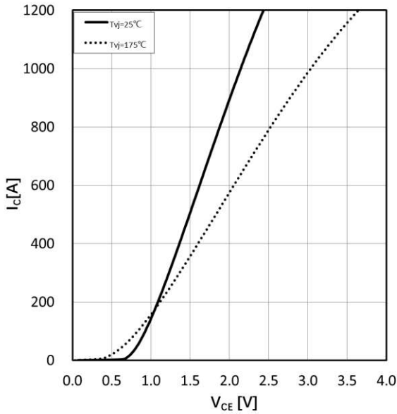
Fig.1 Typical Output Characteristic,IGBT,Inverter I_c = f(V_{CE}) V_{GE} = 15V (terminal)
