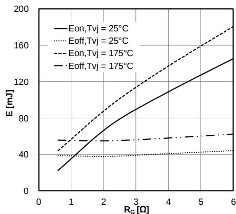
Fig.5 Switching losses, IGBT, Inverter E = f(R_G)
