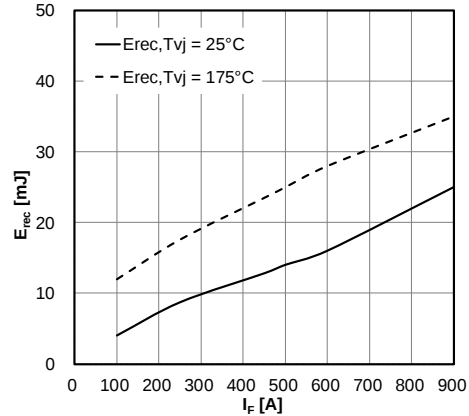
Fig.10 Switching losses, Diode, Inverter
