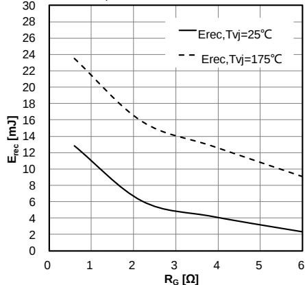
Fig.11 Switching losses, Diode, Inverter
