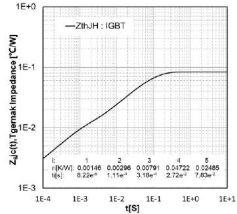
Fig.8 Transient thermal impedance IGBT, Inverter
