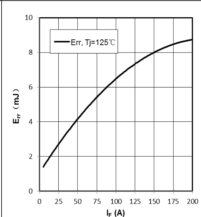
Figure 12. E rr vs I F (Typ) V CC =600V, V GE =+15V/-15V, R G =5.6Ω
