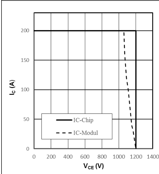
Figure 11. Reverse bias safe operating area IGBT, I C =f(V CE ), V GE =±15V, R Goff =5.6Ω, T vj =125°C
