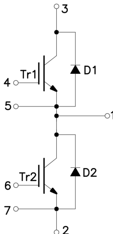
Figure 1. Out drawing & circuit diagram for HCG100FH120A11
