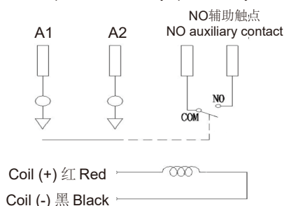
负载无极性，带常开辅助触点 Load non-polar, with normally open auxiliary contact
