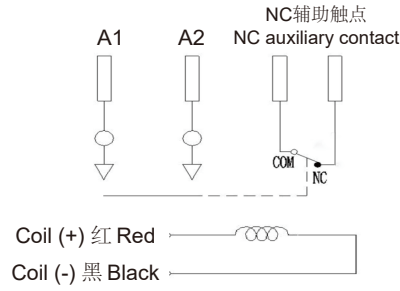
负载无极性，带常闭辅助触点 Load non-polar, with normally closed auxiliary contact
