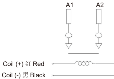
负载无极性，不带辅助 Load non-polar, no auxiliary
