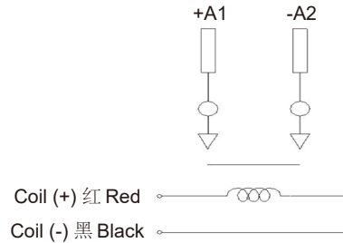
负载有极性，不带辅助 The load is polar, no auxiliary
