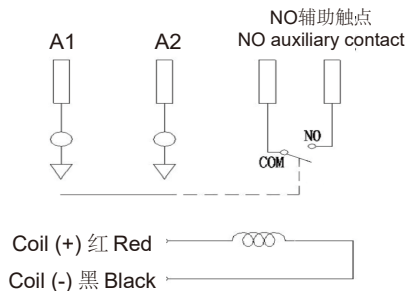
负载无极性，带常开辅助触点 Load non-polar, with normally open auxiliary contact
