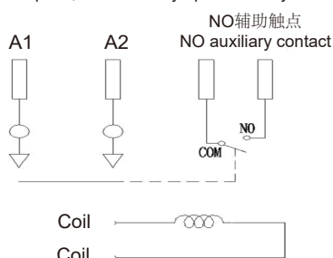
负载无极性，带常开辅助触点 Load non-polar, with normally open auxiliary contact
