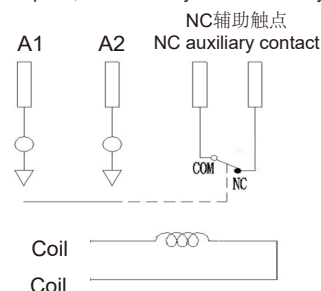
负载无极性，带常闭辅助触点 Load non-polar, with normally closed auxiliary contact
