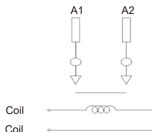
负载无极性，不带辅助 Load non-polar, no auxiliary
