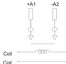
负载有极性，不带辅助 The load is polar, no auxiliary
