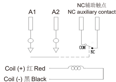
负载无极性, 带常闭辅助触点 Load non-polar, with normally closed auxiliary contact
