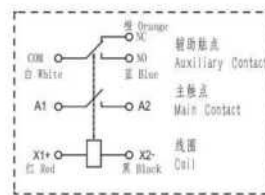
接线图 Coil Wiring Diagram
