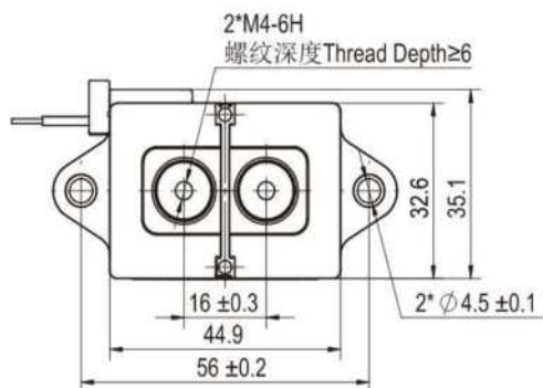
组合螺钉示意 (选配) Combination Screw(Optional)
