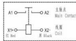
接线图 Coil Wiring Diagram
