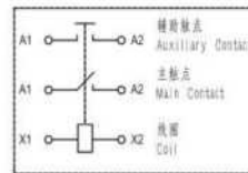
接线图 Coil Wiring Diagram
