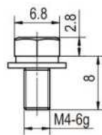
组合螺钉示意 (选配) Combination Screw(Optional)
