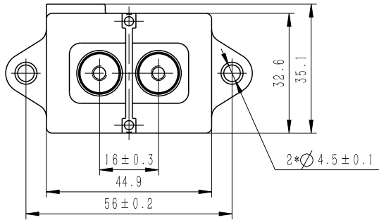
组合螺钉示意(选配) Combination Screw(Optional)
