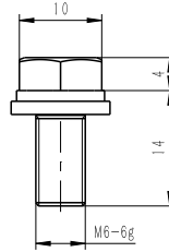
组合螺钉示意(选配) Combination Screw(Optional)
