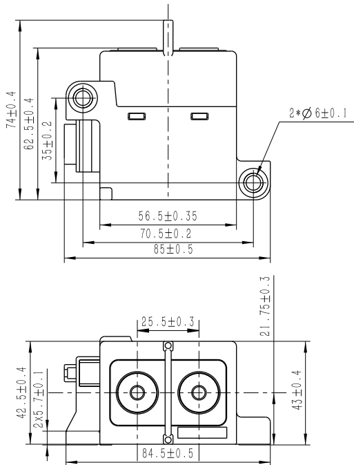
组合螺钉示意(选配) Combination Screw(Optional)
