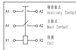
接线图 Coil Wiring Diagram
