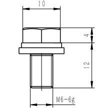
组合螺钉不意(选配) Combination Screw(Optional)
