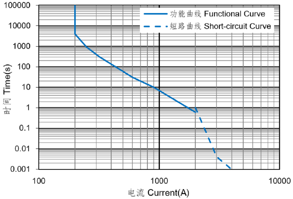
电流承载曲线 Current Carry Curve:
