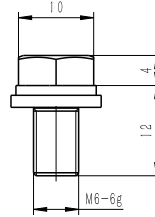
组合螺钉示意(选配) Combination Screw(Optional)
