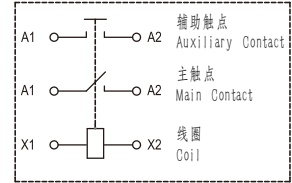
接线图 Coil Wiring Diagram
