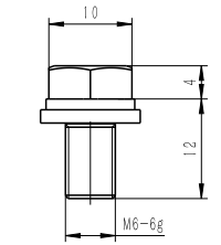
组合螺钉示意(选配) Combination Screw(Optional)
